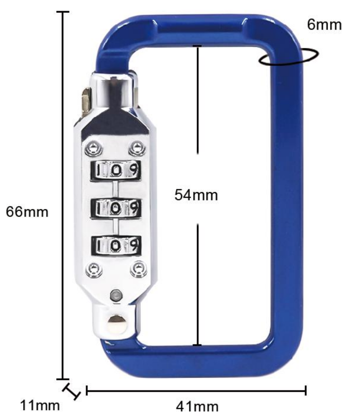
Item:8048 Size: 2.60*1.61*0.43in Material: Zinc alloy Weight: 41g
