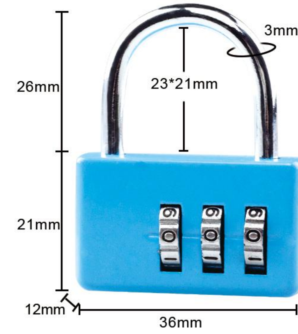
Item:8009 Size: 1.73*1.42*0.47in Material: Zinc alloy Weight: 24g
