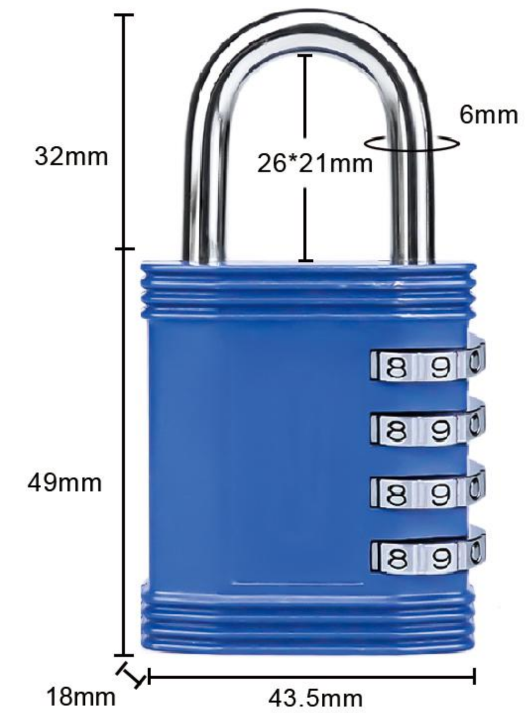
Item:8017A Size: 3.19*1.71*0.71in Material: Zinc alloy Weight: 129.4g
