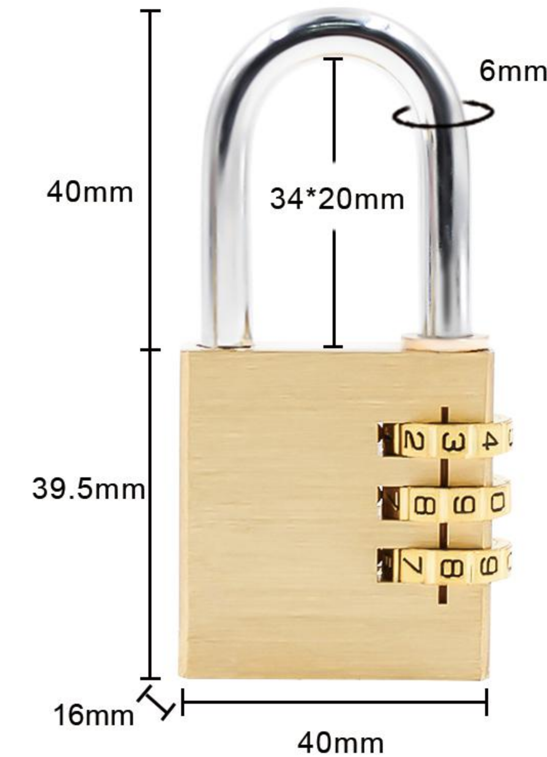
Item:8044 Size: 3.13*1.57*0.63in Material: Brass Weight: 143.3g
