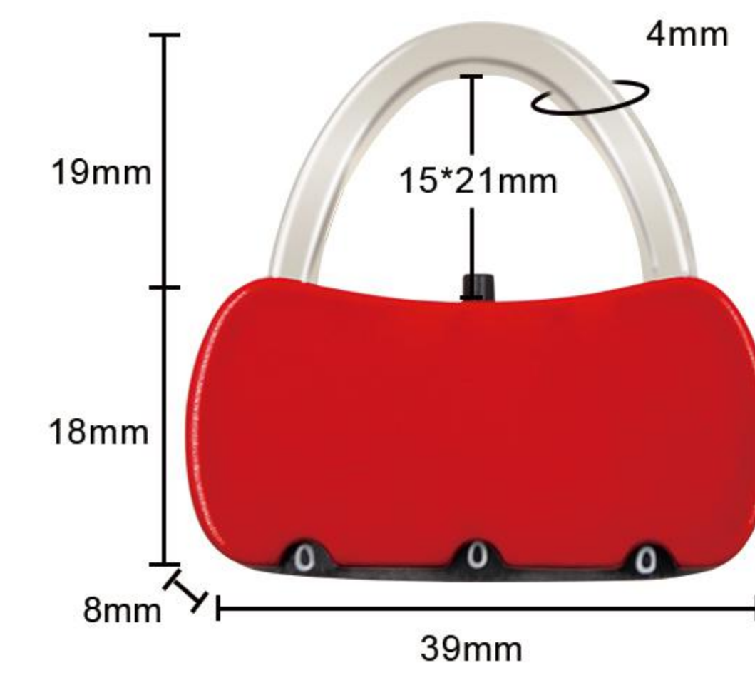
Item:8010 Size: 1.41*1.53*0.35in Material: Zinc alloy Weight: 20.9g
