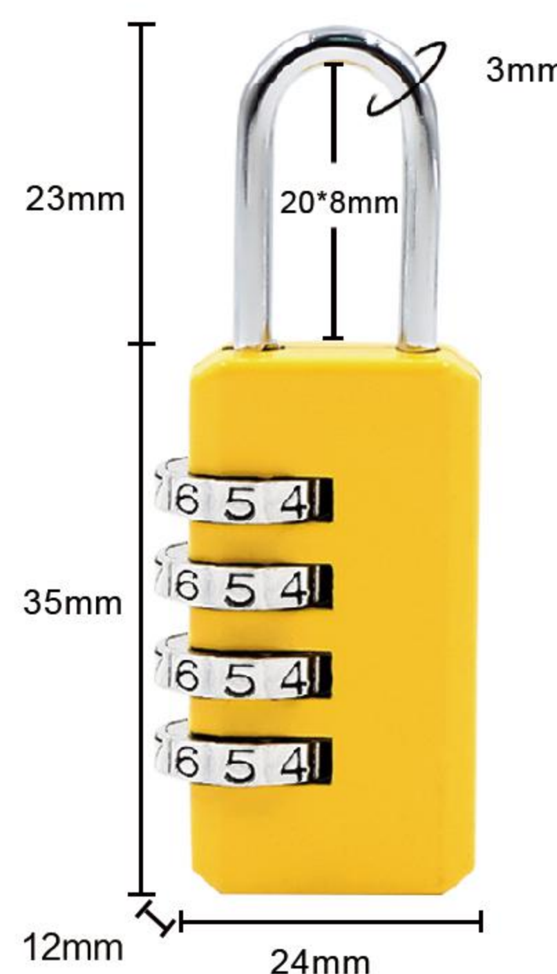
Item:8066 Size: 2.40*0.94*0.47in Material: Zinc alloy Weight: 24g
