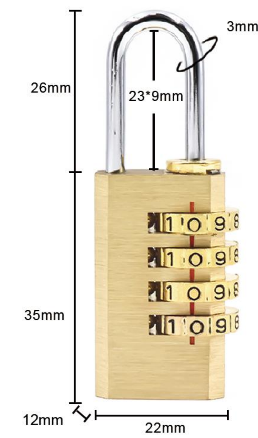
Item:8041 Size: 2.40*0.87*0.53in Material: Brass Weight: 56.5g
