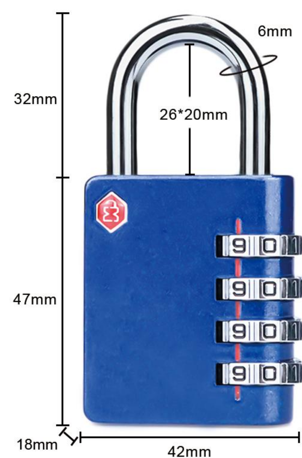
Item:8093 Size: 3.11*1.65*0.71in Material: Zinc alloy Weight: 115g
