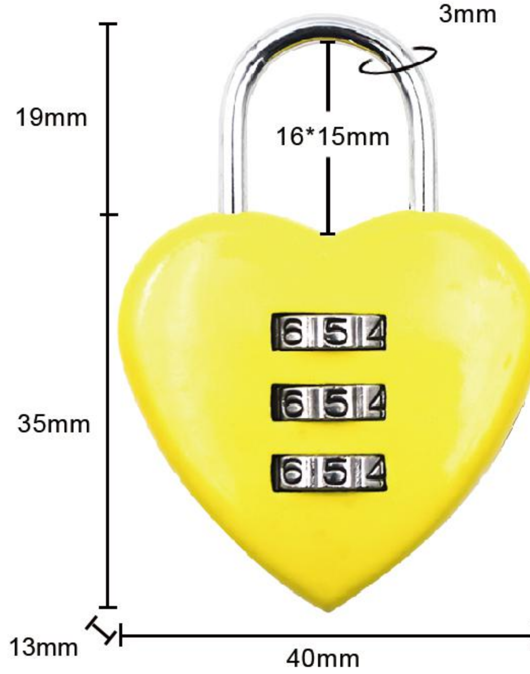
Item:8026 Size: 2.13*1.57*0.51in Material: Zinc alloy Weight: 25.6g
