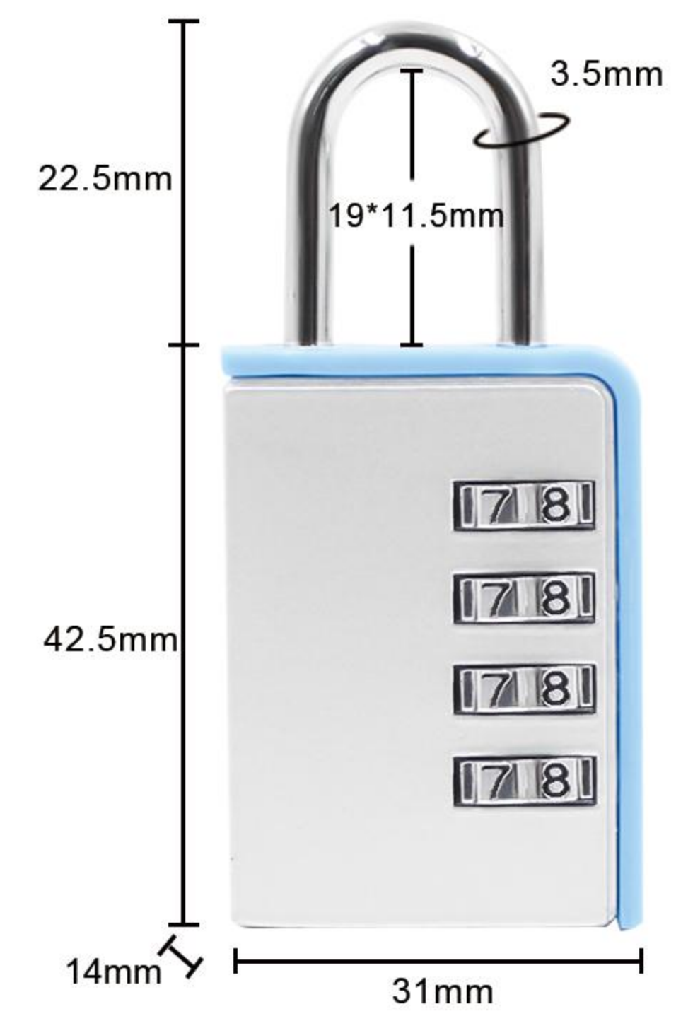
Item:J-8072 Size: 2.56*1.22*0.55in Material: Zinc alloy Weight: 46g
