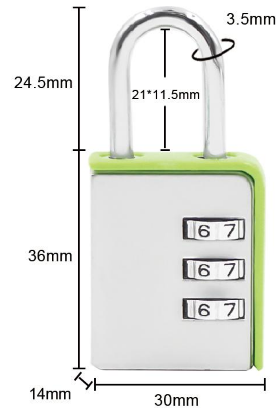
Item:8072S Size: 2.38*1.18*0.55in Material: Zinc alloy Weight: 39g
