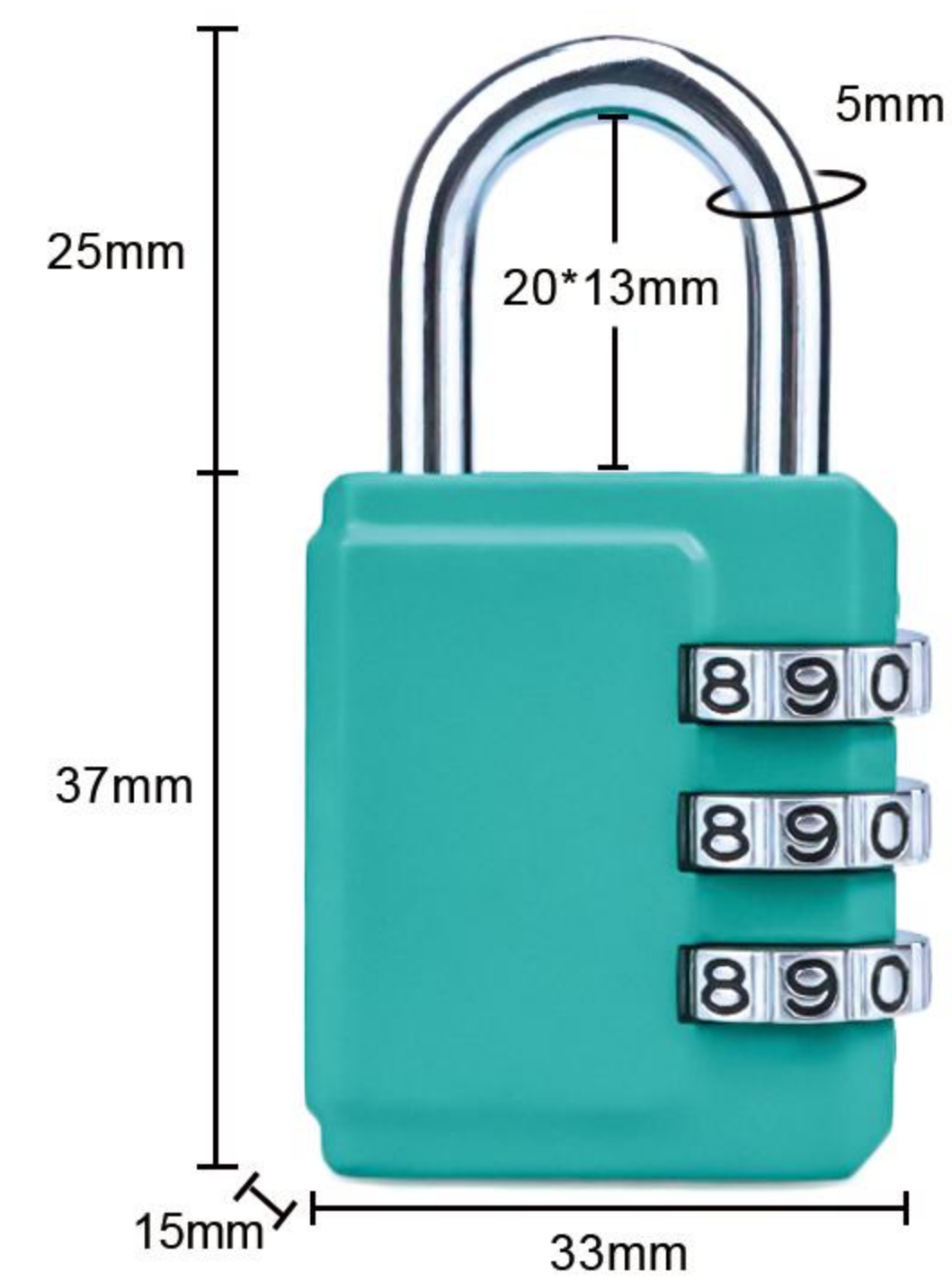
Item:8022A Size: 2.44*1.30*0.59in Material: Zinc alloy Weight: 58g
