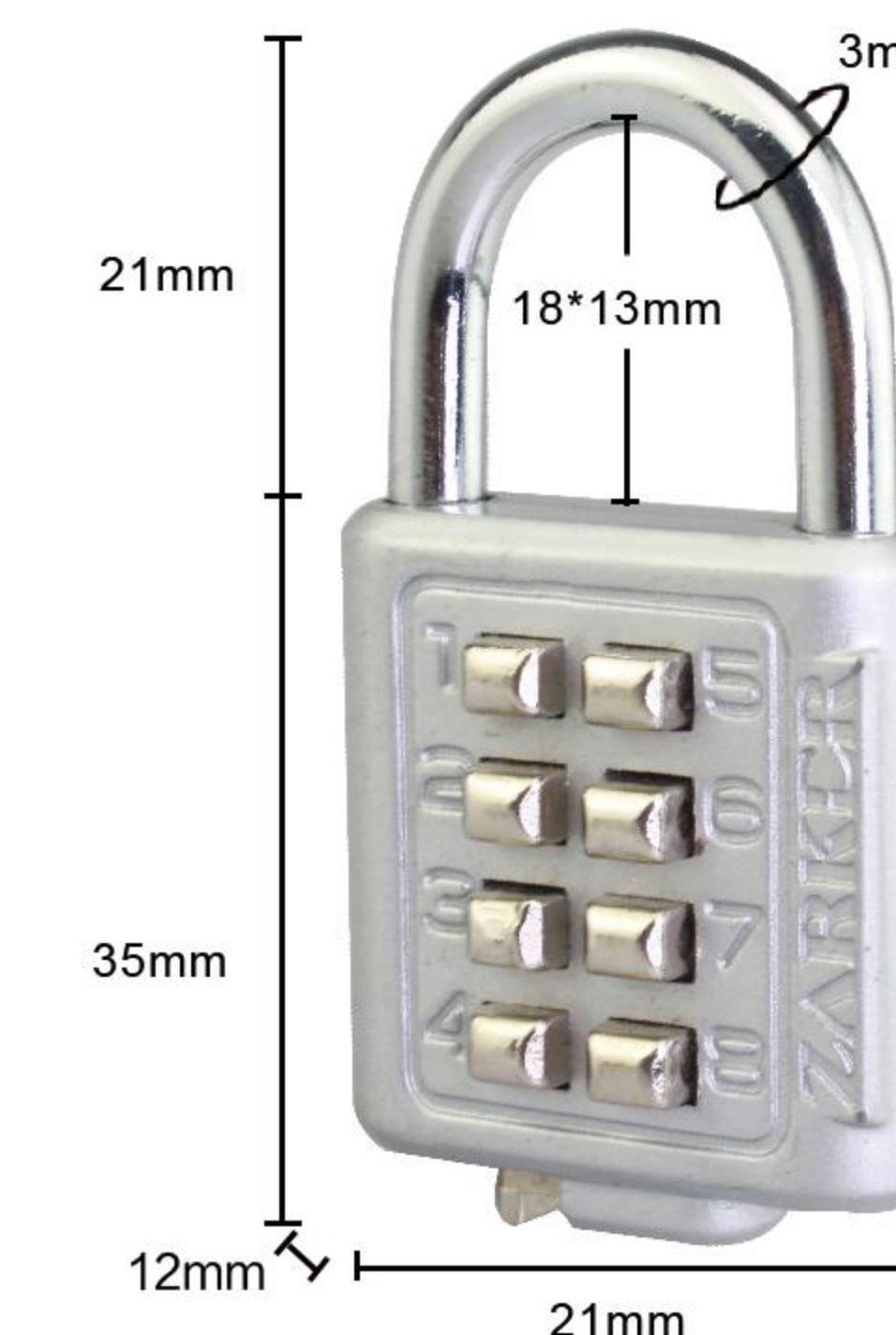
Item:8030 Size: 2.40*0.94*0.39in Material: Zinc alloy Weight: 15g
