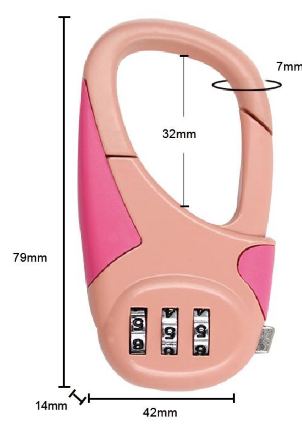
Item:8054 Size: 3.11*1.65*0.55in Material: Zinc alloy Weight: 64.1g
