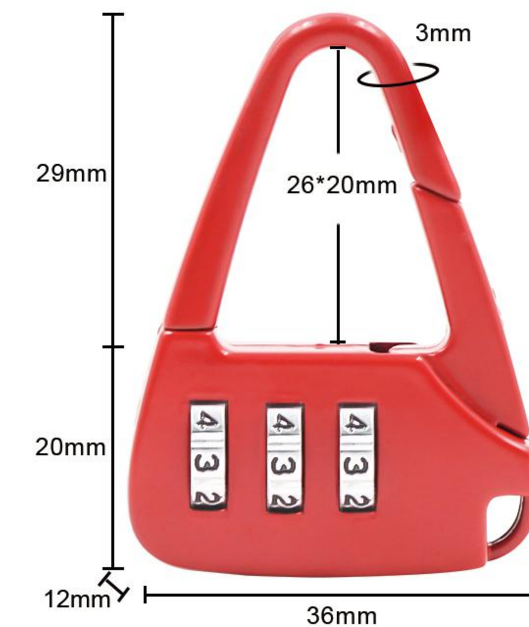
Item:8013 Size: 1.93*1.41*0.47in Material: Zinc alloy Weight: 23.2g
