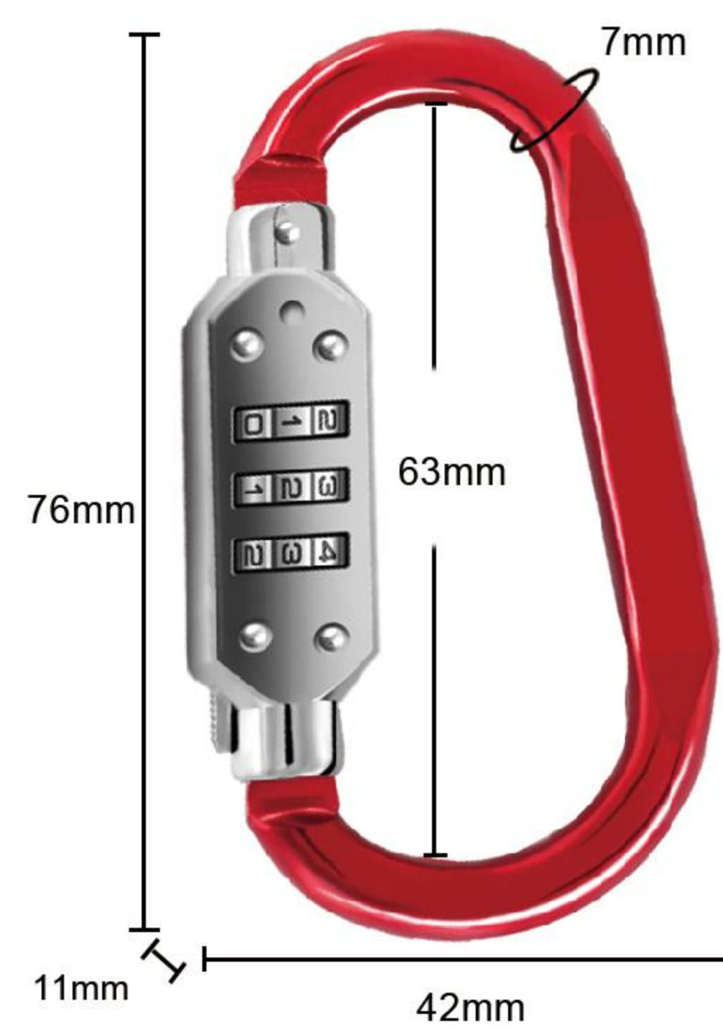
Item:8047 Size: 2.99*1.65*0.43in Material: Zinc alloy Weight: 32g
