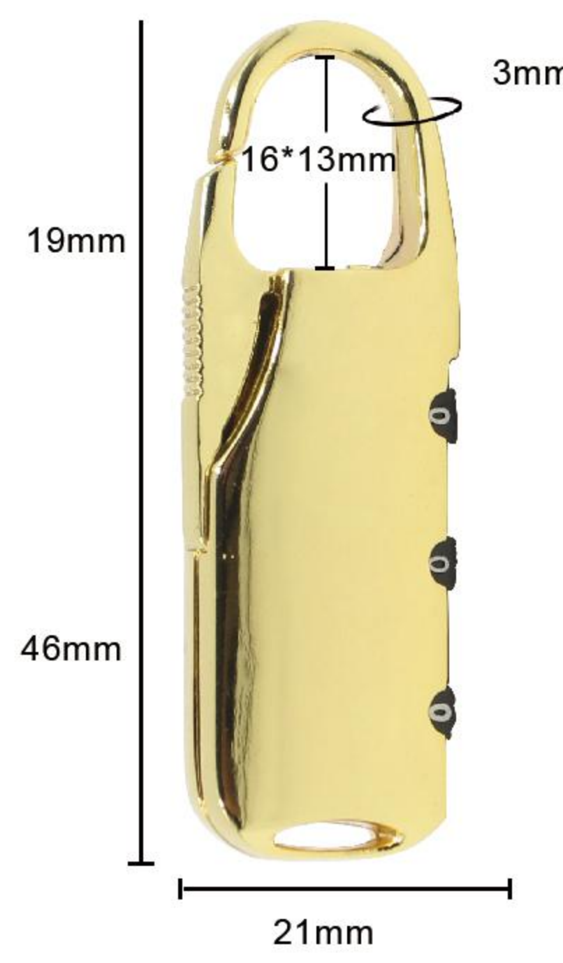
Item:8064A Size: 2.55*0.82*0.35in Material: Zinc alloy Weight: 29g
