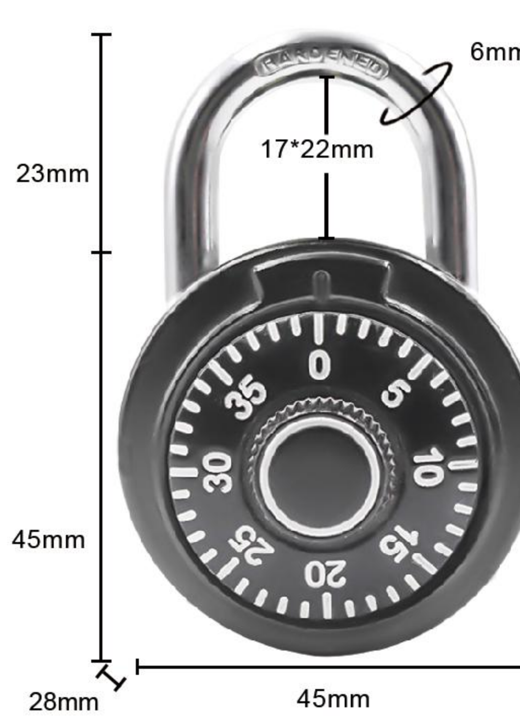
Item:8056B Size: 2.68*1.77*1.10in Material: Zinc alloy Weight: 85g
