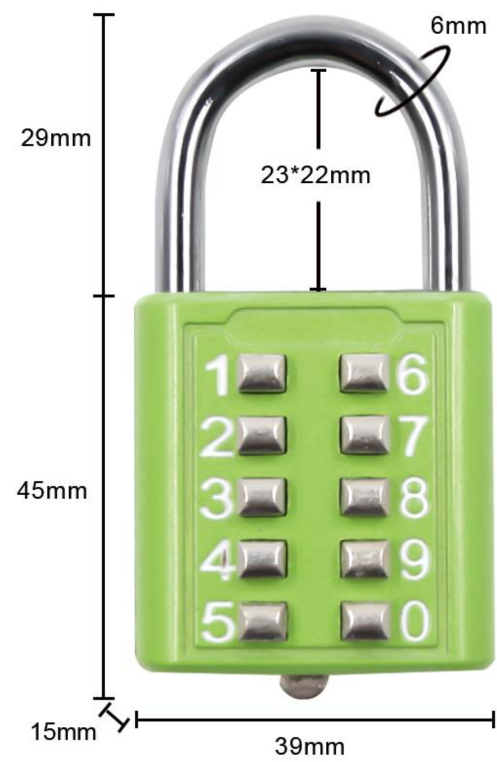
Item:8031A Size: 2.91*1.53*0.59in Material: Zinc alloy Weight: 78g
