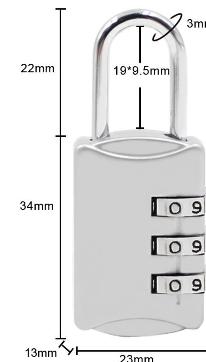
Item:8019 Size: 2.20*0.90*0.51in Material: Zinc alloy Weight: 25.1g
