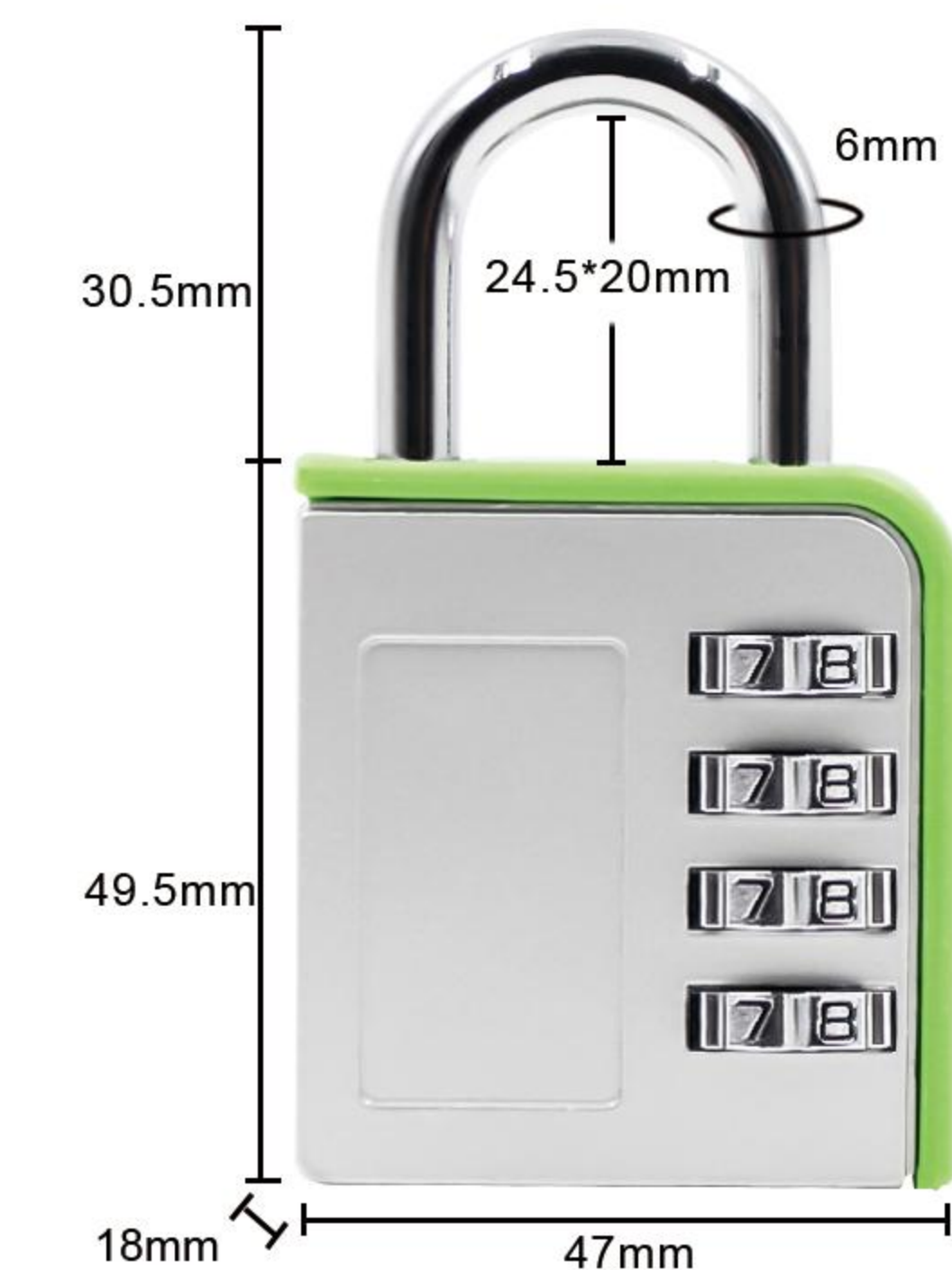
Item:8072L Size: 3.15*1.85*0.71in Material: Zinc alloy Weight: 119g
