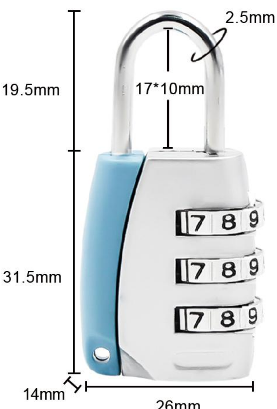
Item:8075 Size: 2.00*1.02*0.55in Material: Zinc alloy Weight: 28.4g
