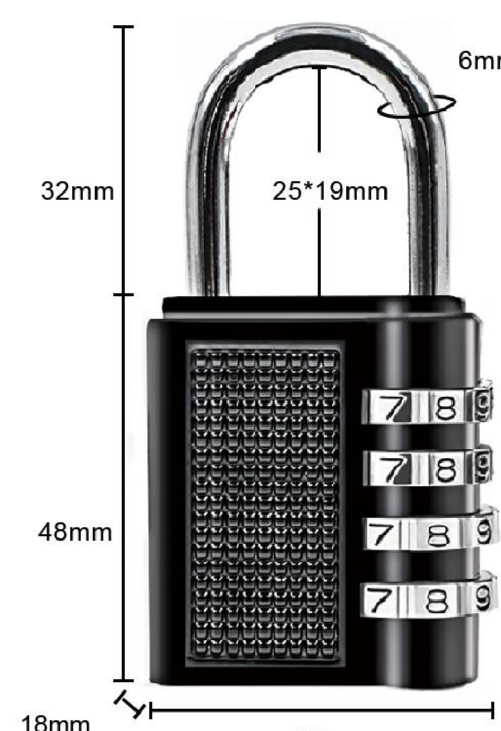
Item:8024 Size: 3.15*1.65*0.71in Material: Zinc alloy Weight: 102.2g
