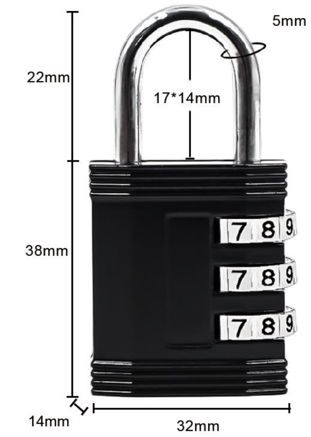
Item:8017 Size: 2.36*1.26*0.55in Material: Zinc alloy Weight: 60.2g
