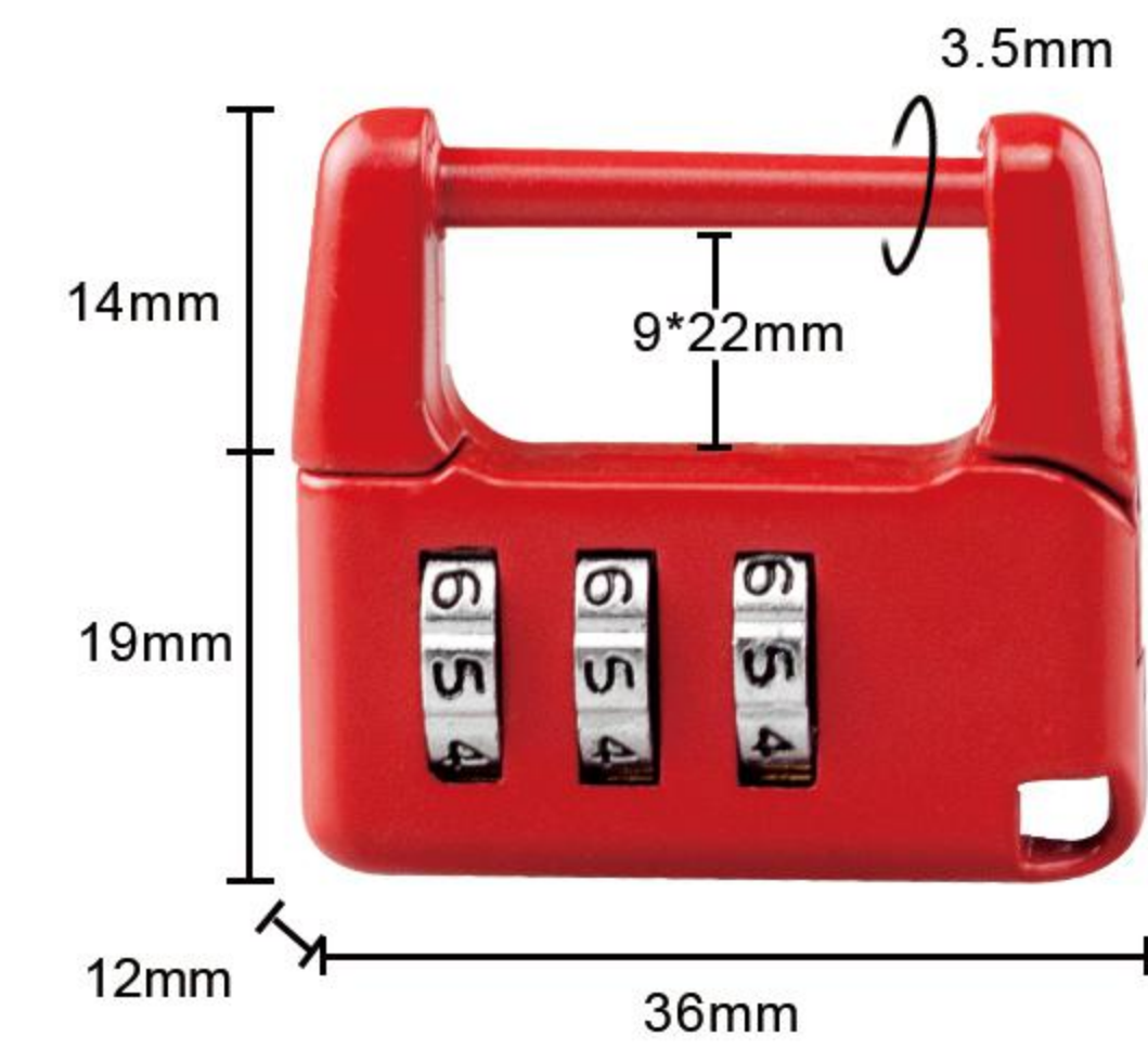
Item:8008 Size: 1.30*1.42*0.47in Material: Zinc alloy Weight: 19.5g
