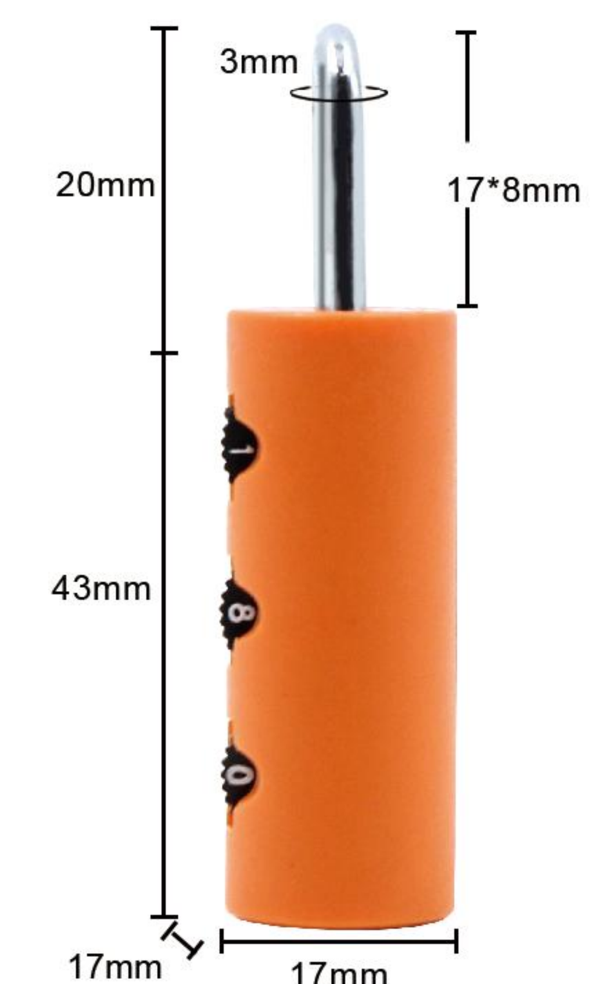
Item:8029 Size: 2.40*0.67*0.67in Material: ABS plastic Weight: 8.6g
