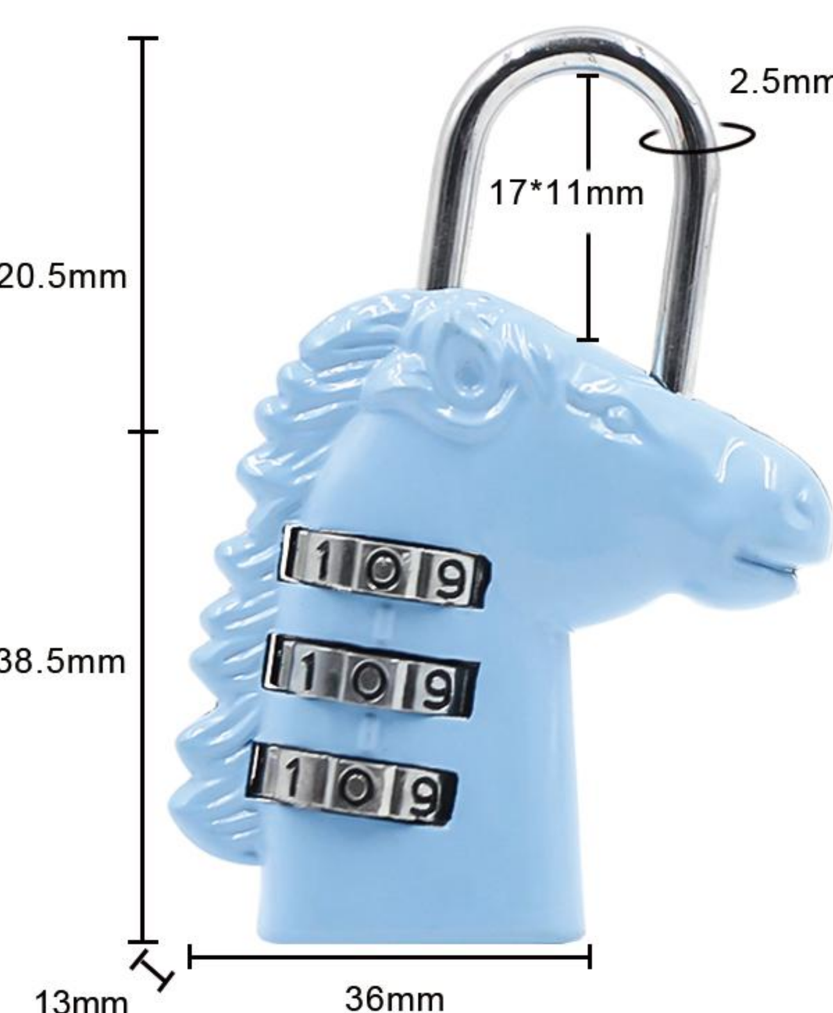
Item:8061 Size: 2.32*1.42*0.51in Material: Zinc alloy Weight: 24.8g
